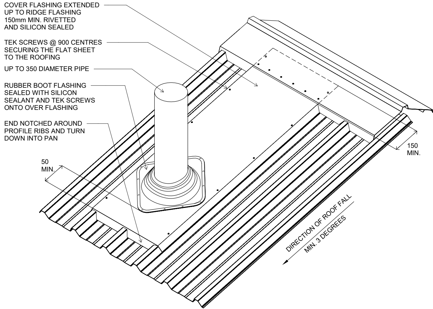
P PIPE PENETRATION DETAIL CAD REF: ROOF\SPD-VEEDEK
