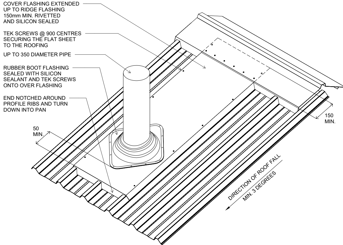
P PIPE PENETRATION DETAIL CAD REF: ROOFHI-FIVE
