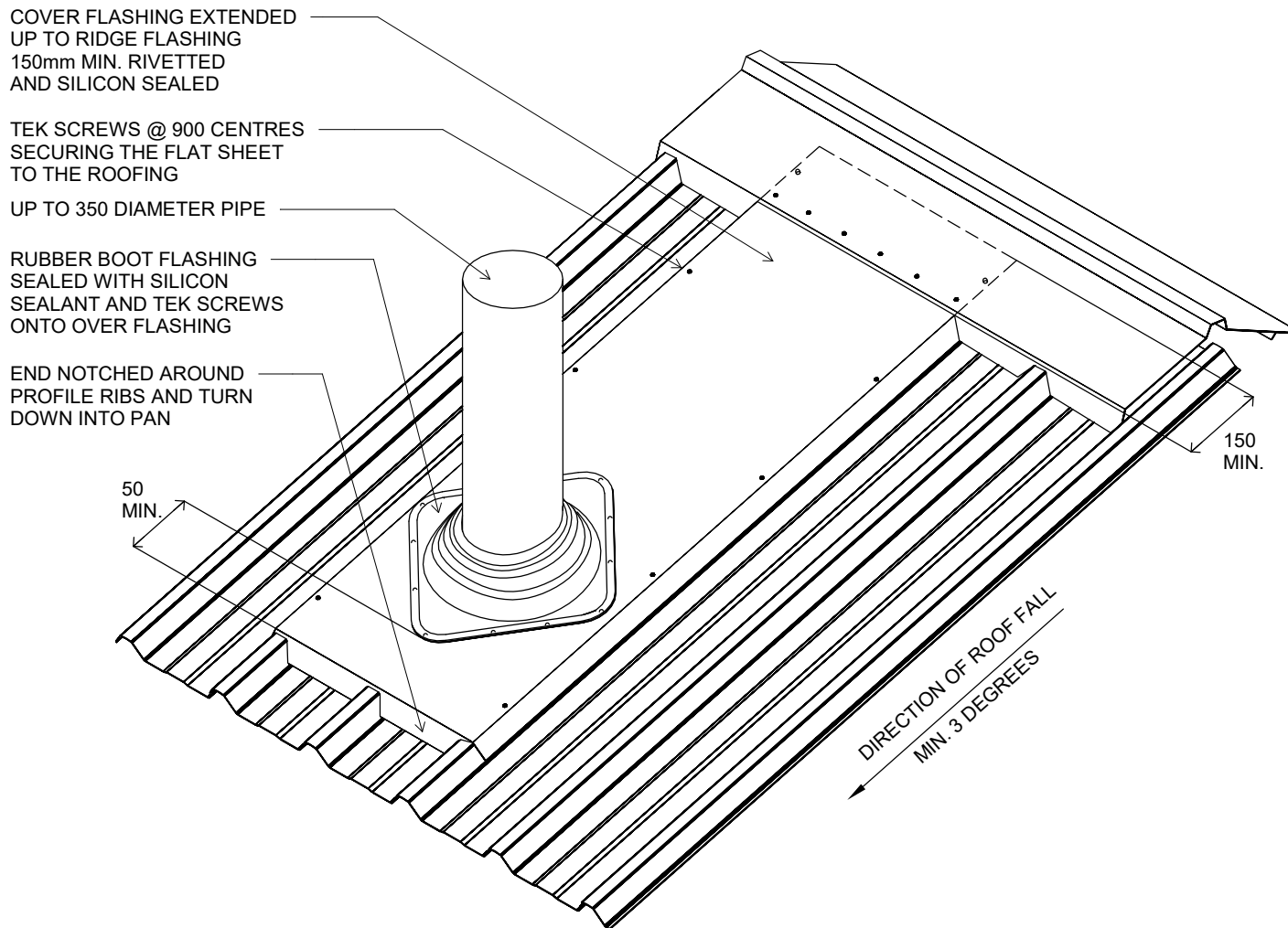
P PIPE PENETRATION DETAIL . CAD REF: ROOF\SOLAR RIB
