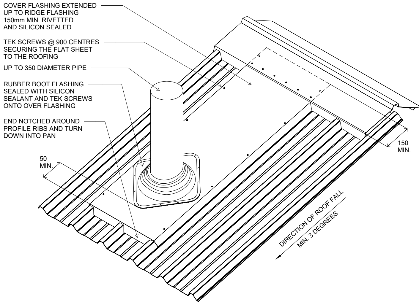
P PIPE PENETRATION DETAIL CAD REF: ROOF\SPD-STYLELINE
