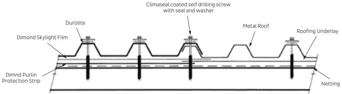
Fig 1 Dimond Skylight Film Detail
