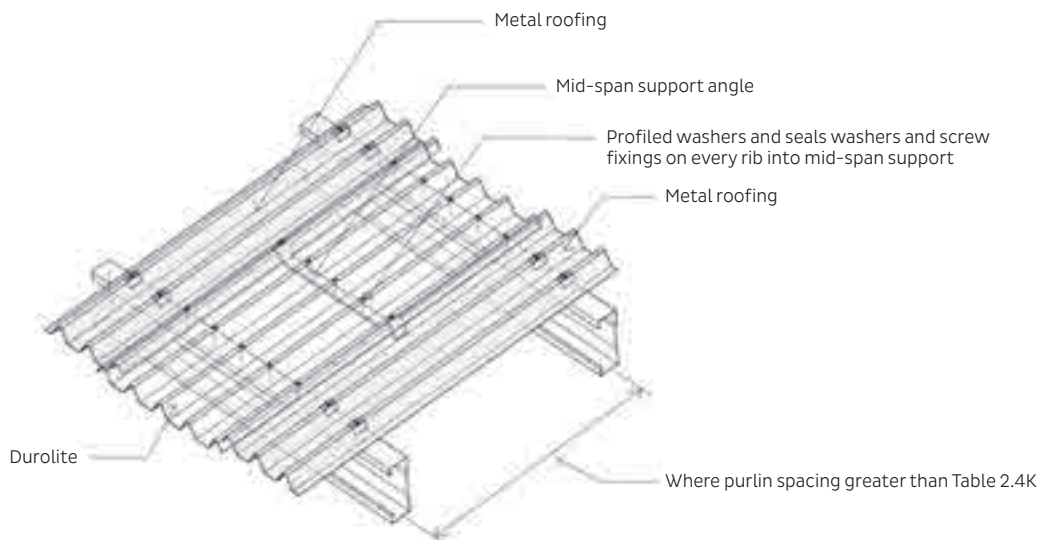
Fig 12 Mid-Span Support Detail (All Profiles Except Decking)
