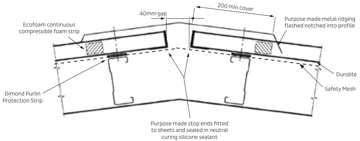
Fig 3 Detail At Ridge
