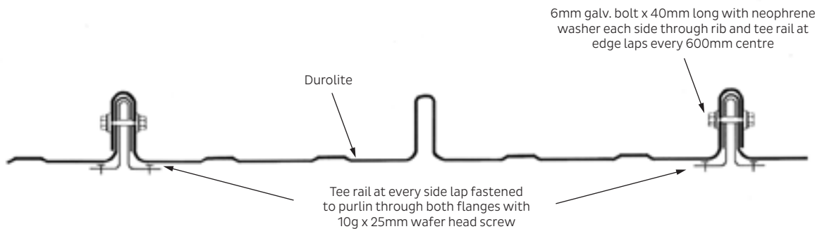
Fig 9 Multiple Durolite Sheet Detail With Dimondek® 300 or Dimondek® 400
